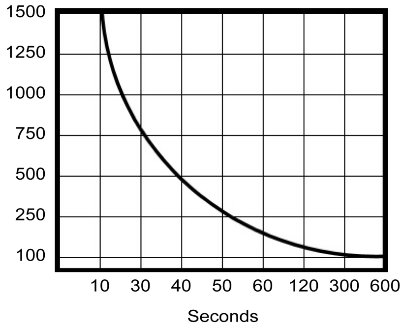
Power Capability
