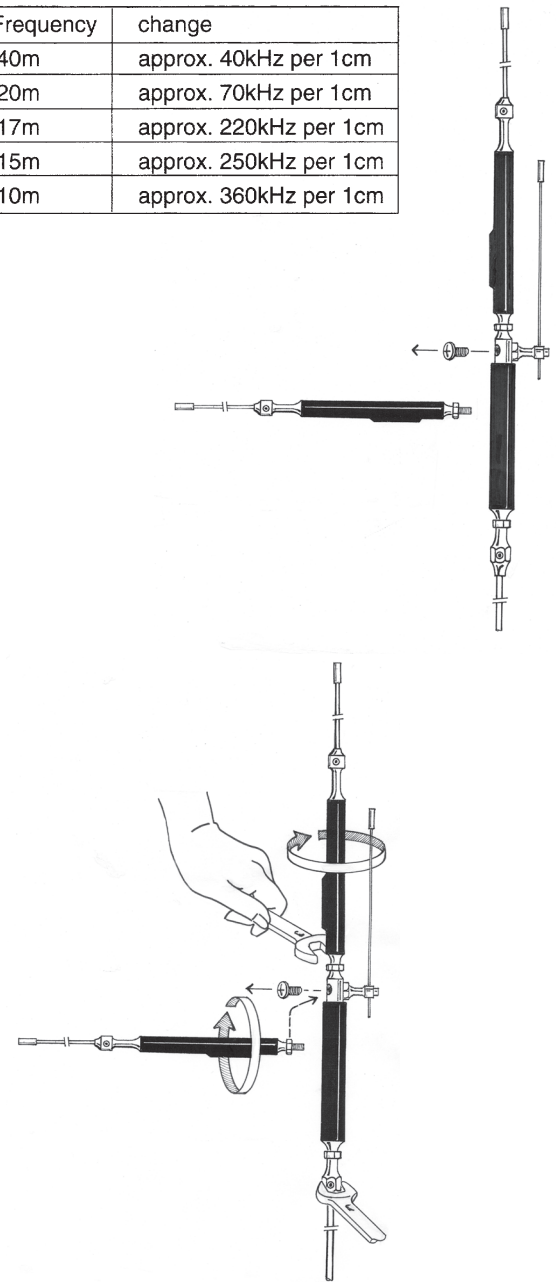
Adjustment element length vs. frequency change on each frequency band.
