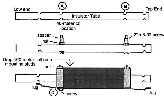
FIG-4: Mounting Loading Coil
