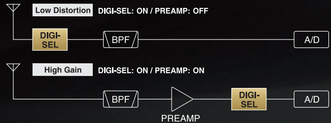
■ Block Diagram Overview
